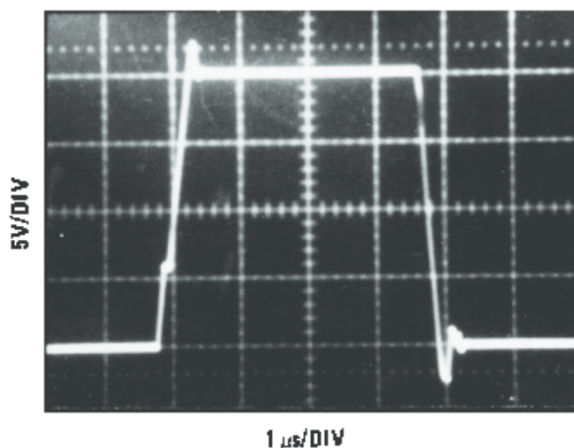
Figure 38. LF357
